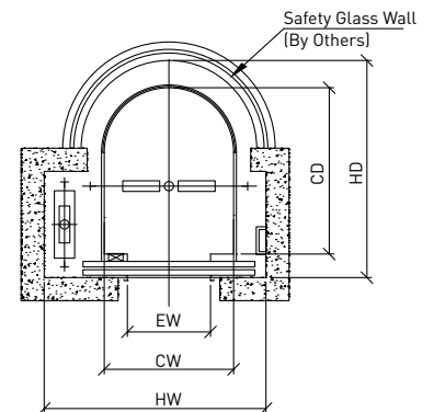
SHAFT PLAN
