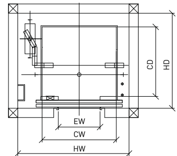
SHAFT PLAN
