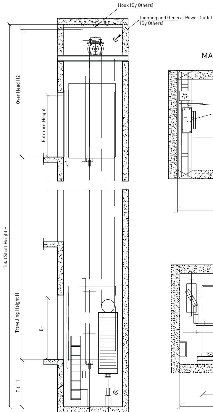
SHAFT SECTION
