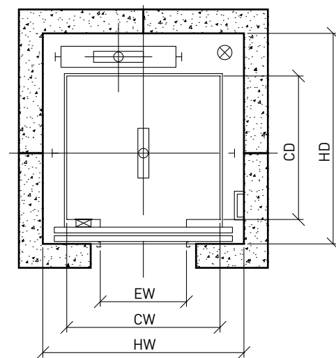
SHAFT PLAN
