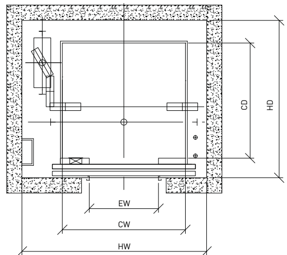
SHAFT PLAN
