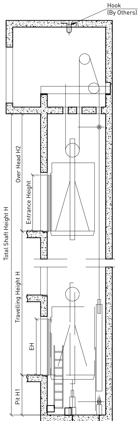
SHAFT SECTION
