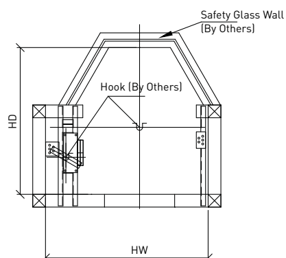
MACHINE ROOM PLAN
