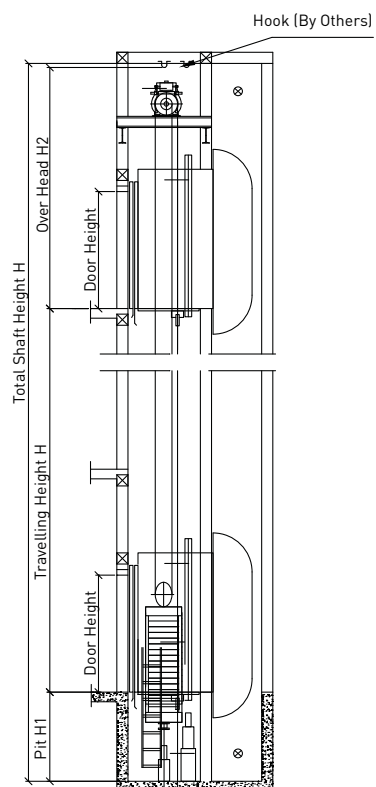
SHAFT SECTION
