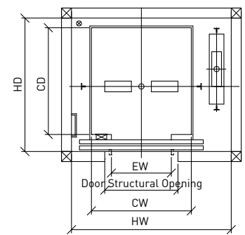
SHAFT PLAN
