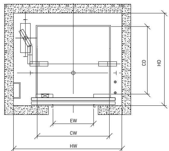
SHAFT PLAN
